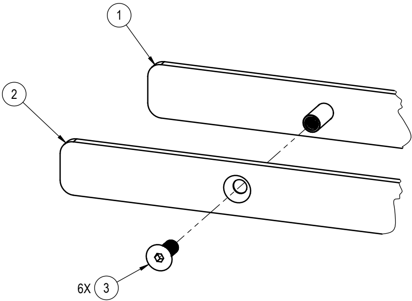
DETAIL C SCALE 2 : 5
