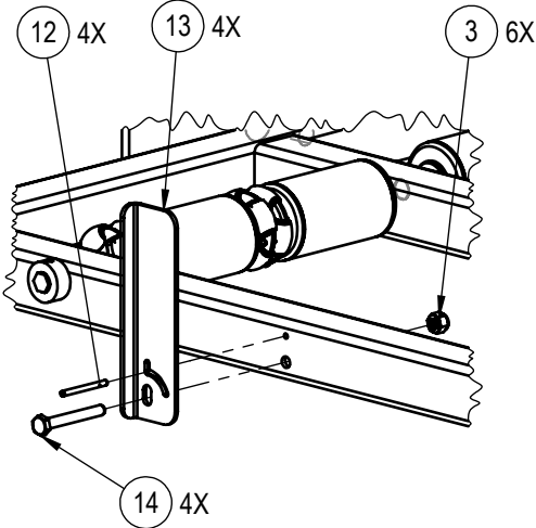
SHEET METAL FLIP LATCH ASSEMBLY DETAIL SCALE 1: 5
