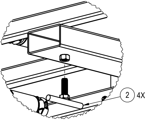
SAFETY BOLT ASSEMBLY SCALE 1:5
